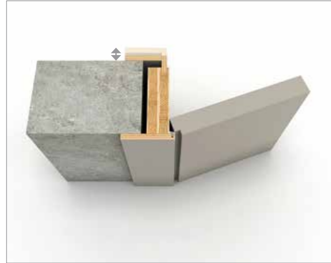
FLUSH FRAME 01 IN
