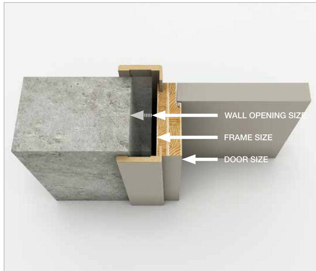
Important measures for standard swing doors
